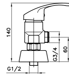
Basin Mixer
