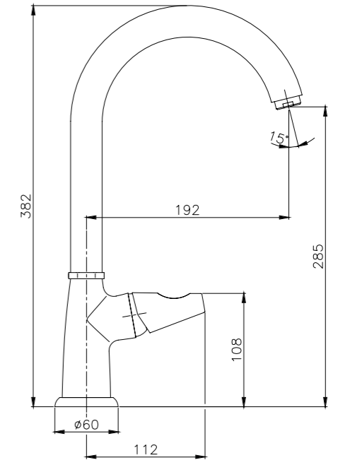
Kitchen Mixer
