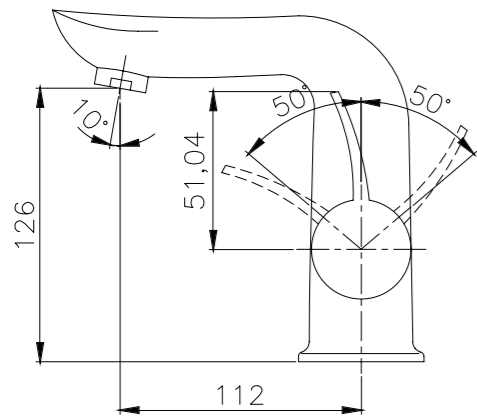
Basin Mixer
