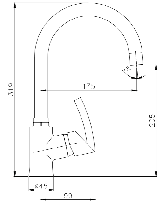
Kitchen Mixer
