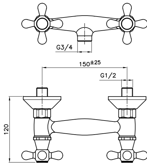
Basin Mixer
