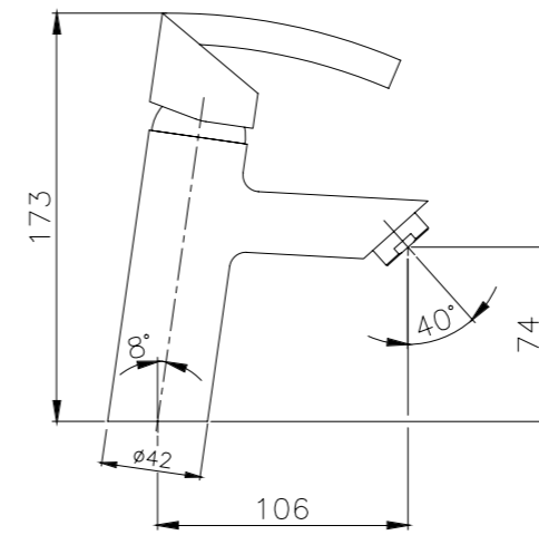
Basin Mixer
