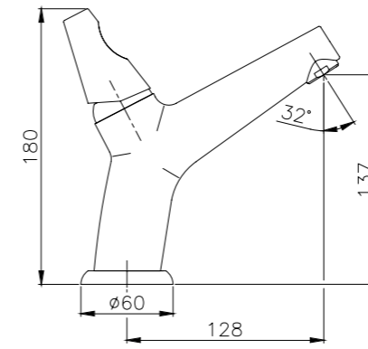
Basin Mixer
