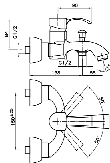
Bath Mixer
