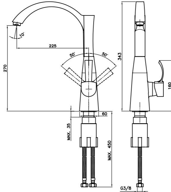
Kitchen Mixer
