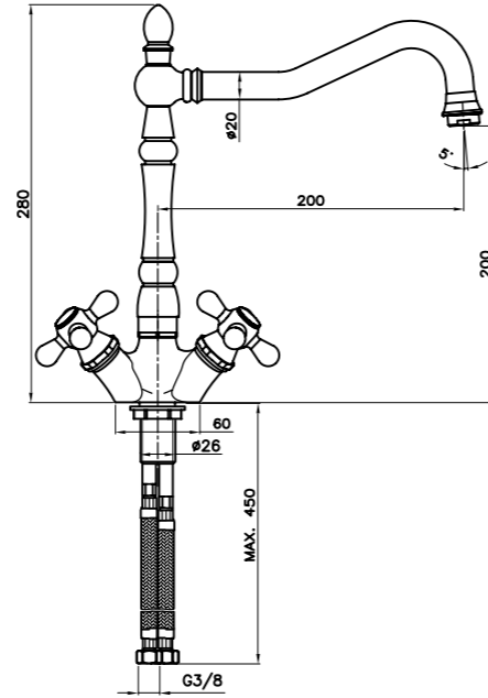
Kitchen Mixer
