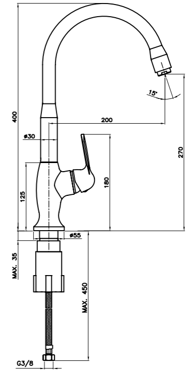
Kitchen Mixer
