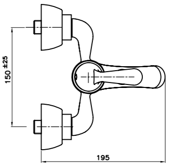
Bath Mixer
