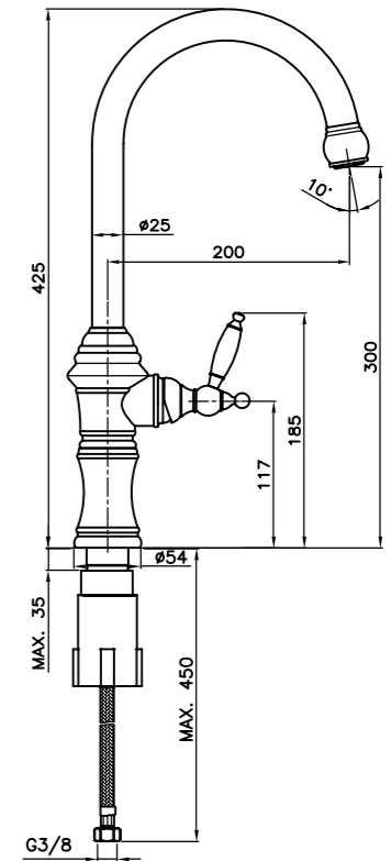
Kitchen Mixer
