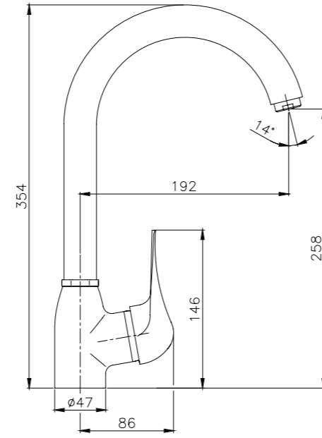
Kitchen Mixer
