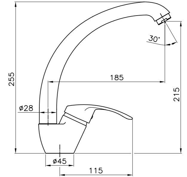
Kitchen Mixer
