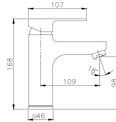
Basin Mixer
