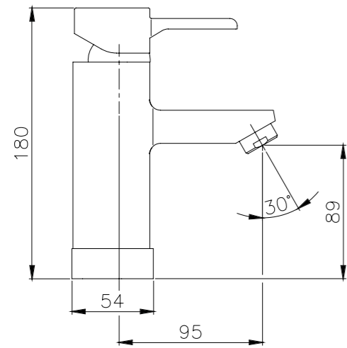
Basin Mixer
